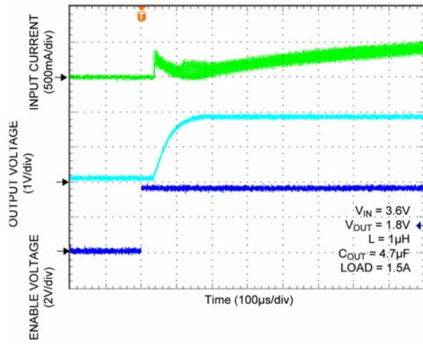
Turn-On Time
