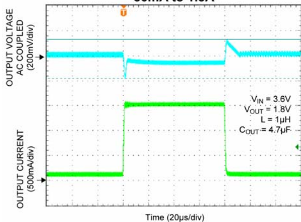
Load Transient 50mA to 1.5A
